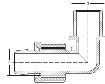
YASSI - ERKEK DİRSEK TAPE - MALE ELBOW
