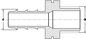
KURTAĞZI - ERKEK NİPEL BARBED - MALE NIPPLE
