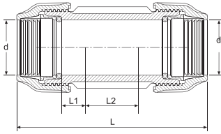
TAMİR MANŞONU REPAIRING COUPLING
